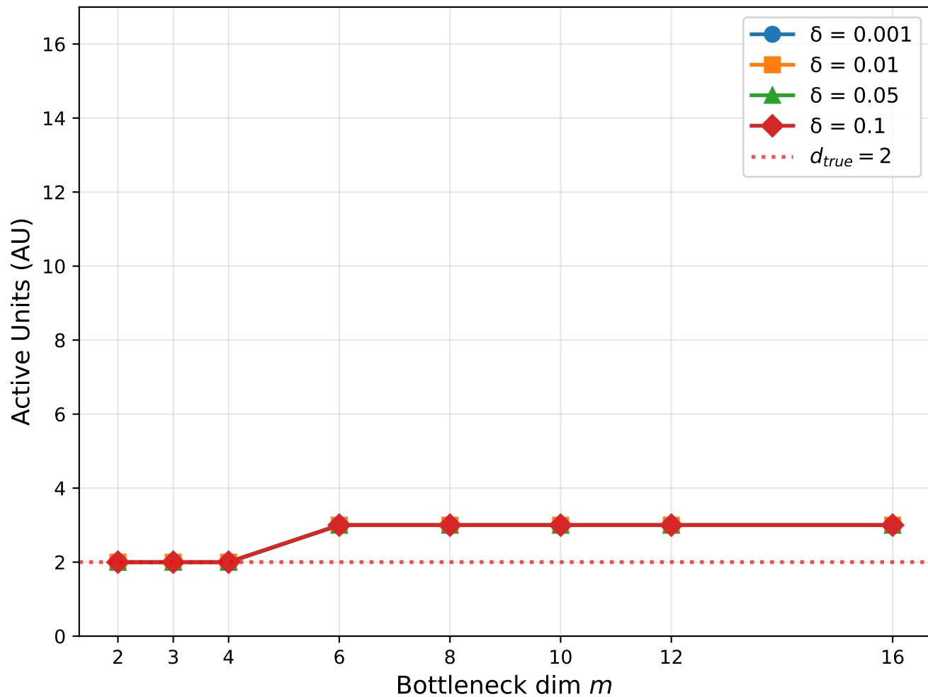
Torus ( d_{true} = 2 )
