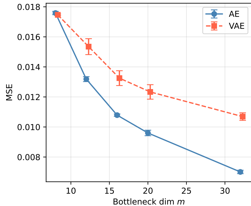
MNIST MSE (mean \pm std, 3 seeds)
