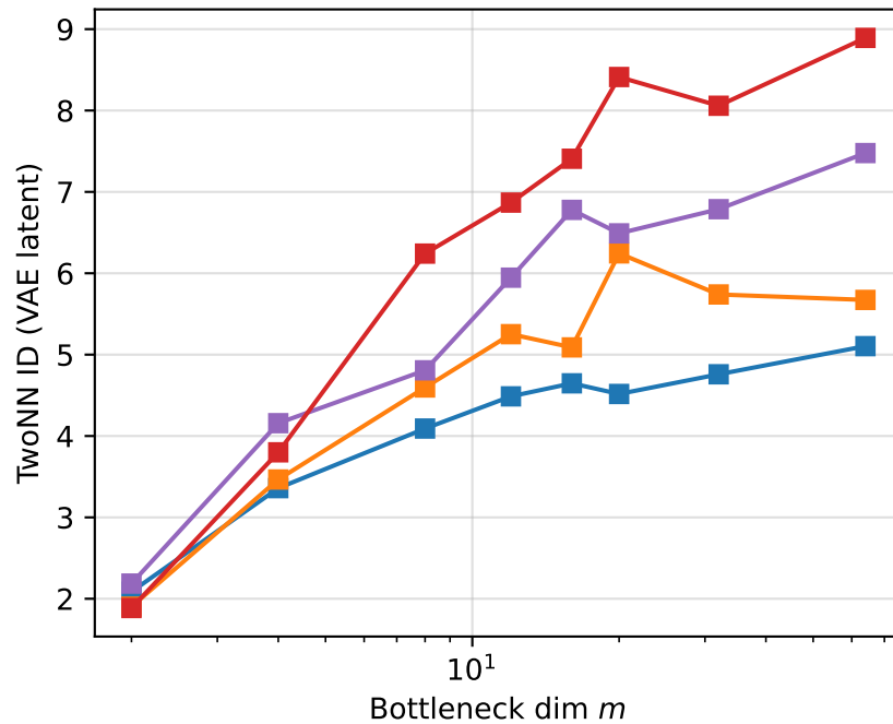
TwoNN ID vs m
