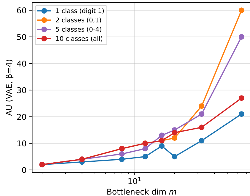
AU vs m by class count
