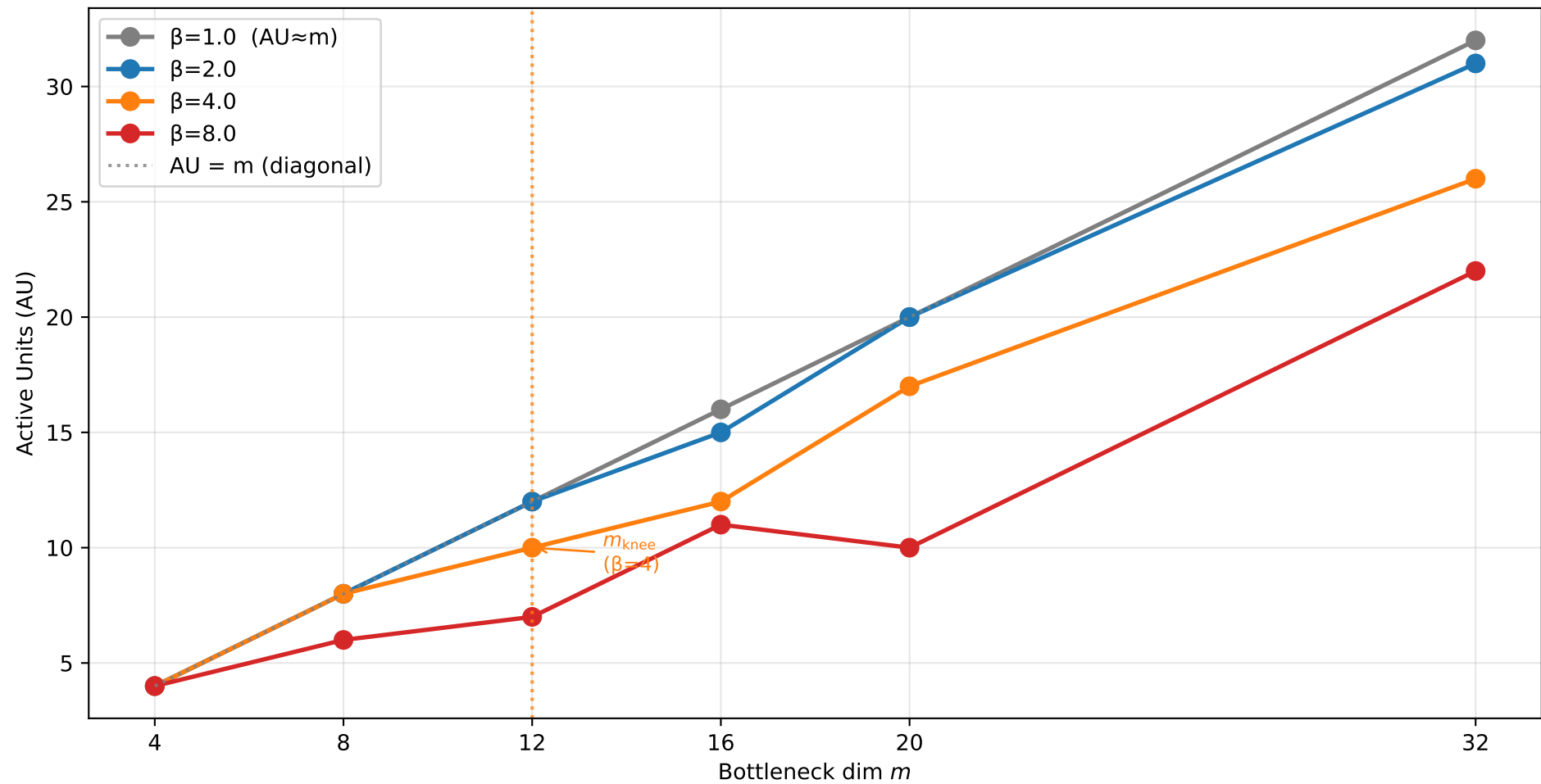
\beta -sensitivity: MNIST VAE AU( m ) (50ep, n=5,000 subset)
