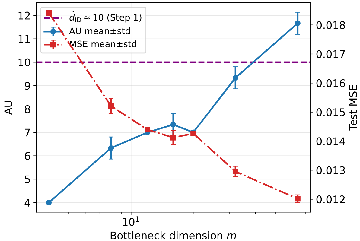
Mean \pm std over 3 seeds (Fashion-MNIST)
