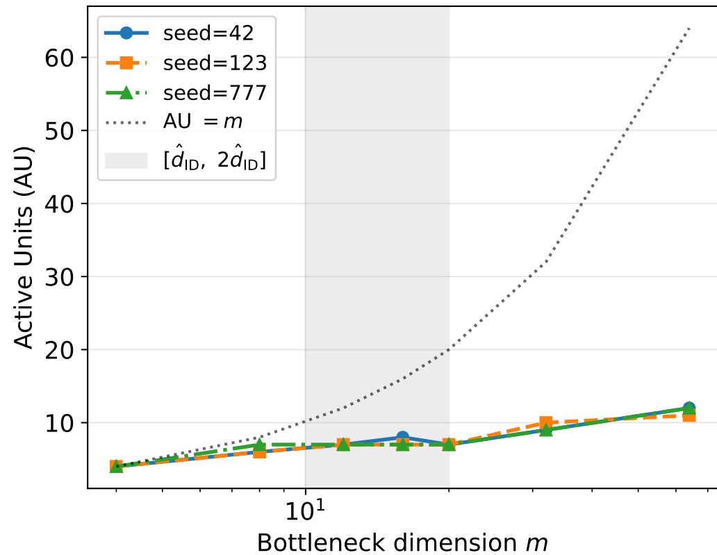
Fashion-MNIST FC-VAE: AU vs. m (3 seeds, 300 ep)
