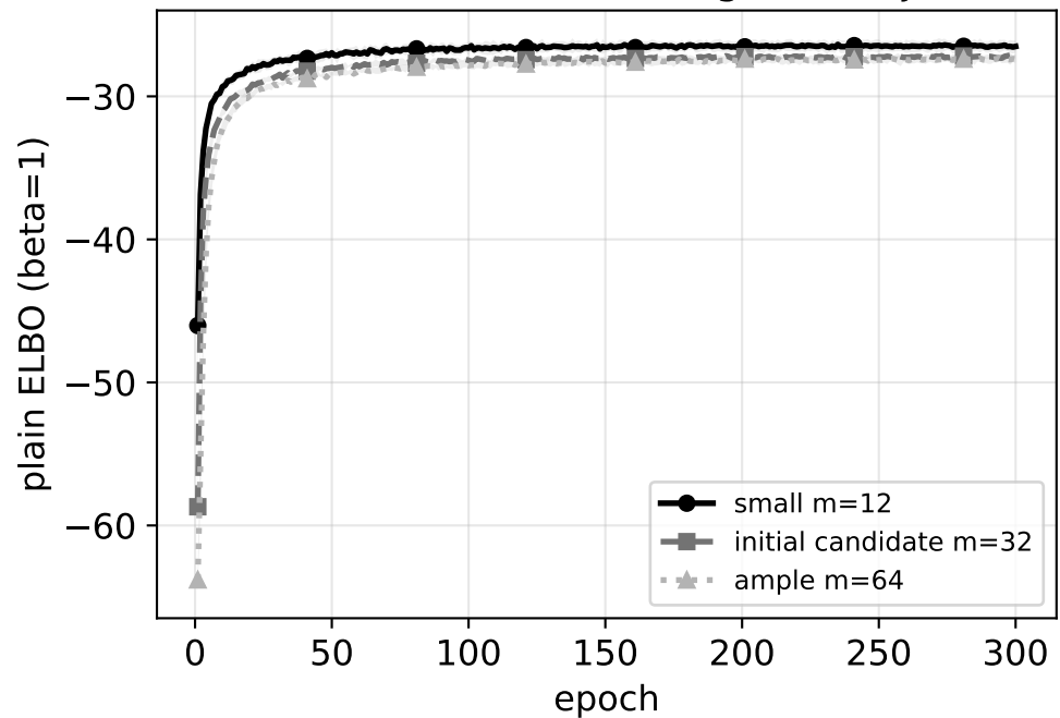
MNIST: plain ELBO (distinct from the beta-weighted objective)
