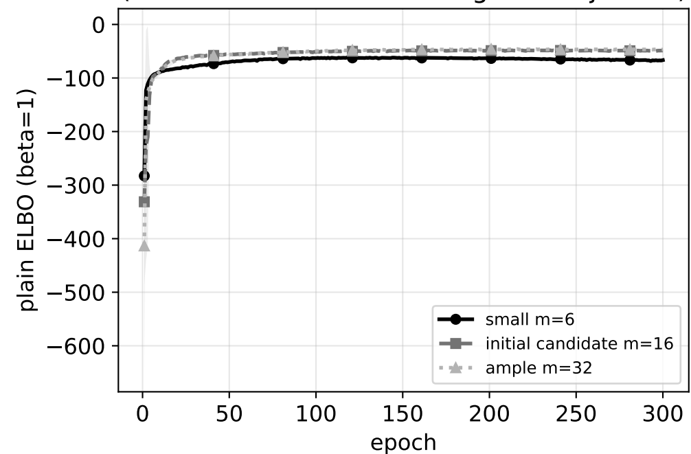
dSprites: plain ELBO (distinct from the beta-weighted objective)
