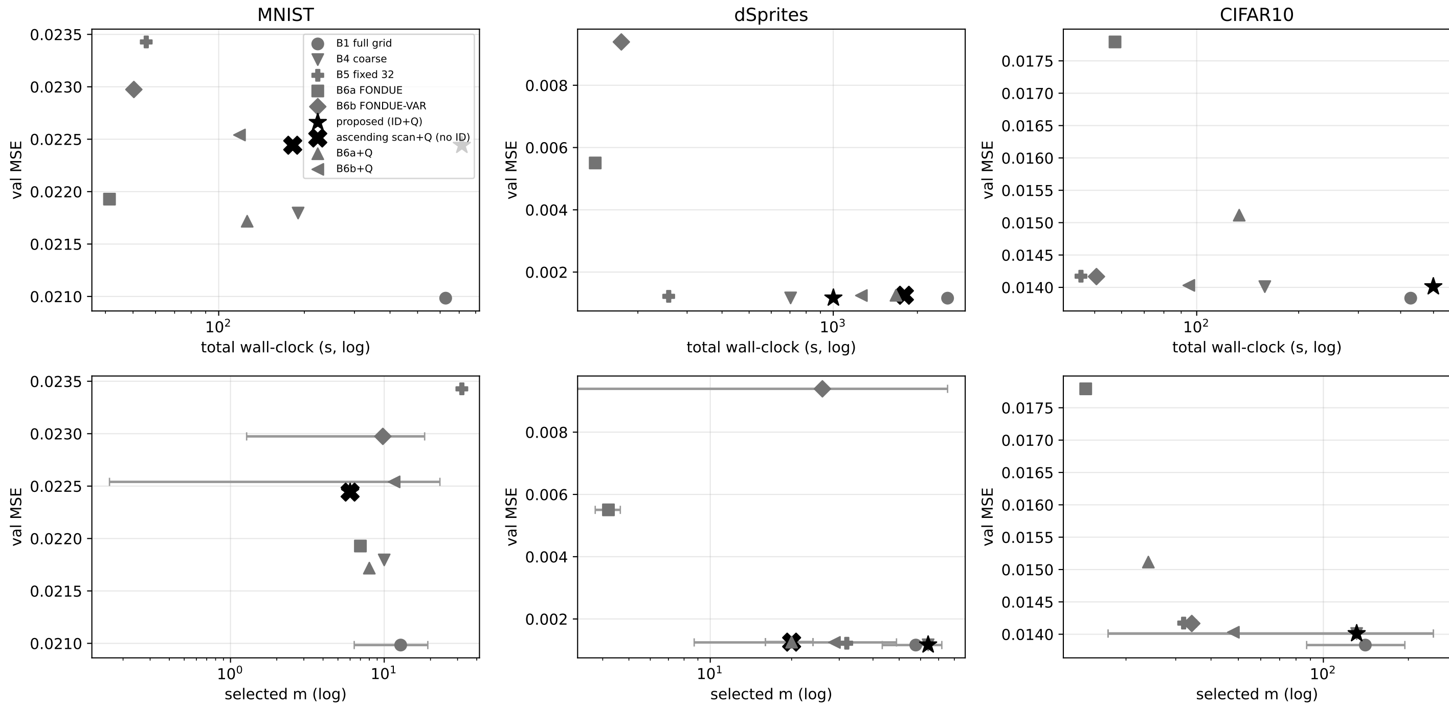
Figure B: quality vs cost (top) and quality vs selected dimension (bottom) beta=1, 5 seeds; error bars are SD of the selected m across seeds
