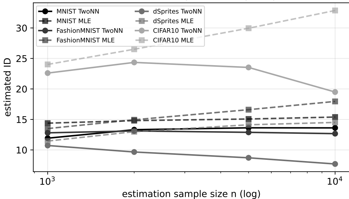
ID estimate vs sample size (input space)
