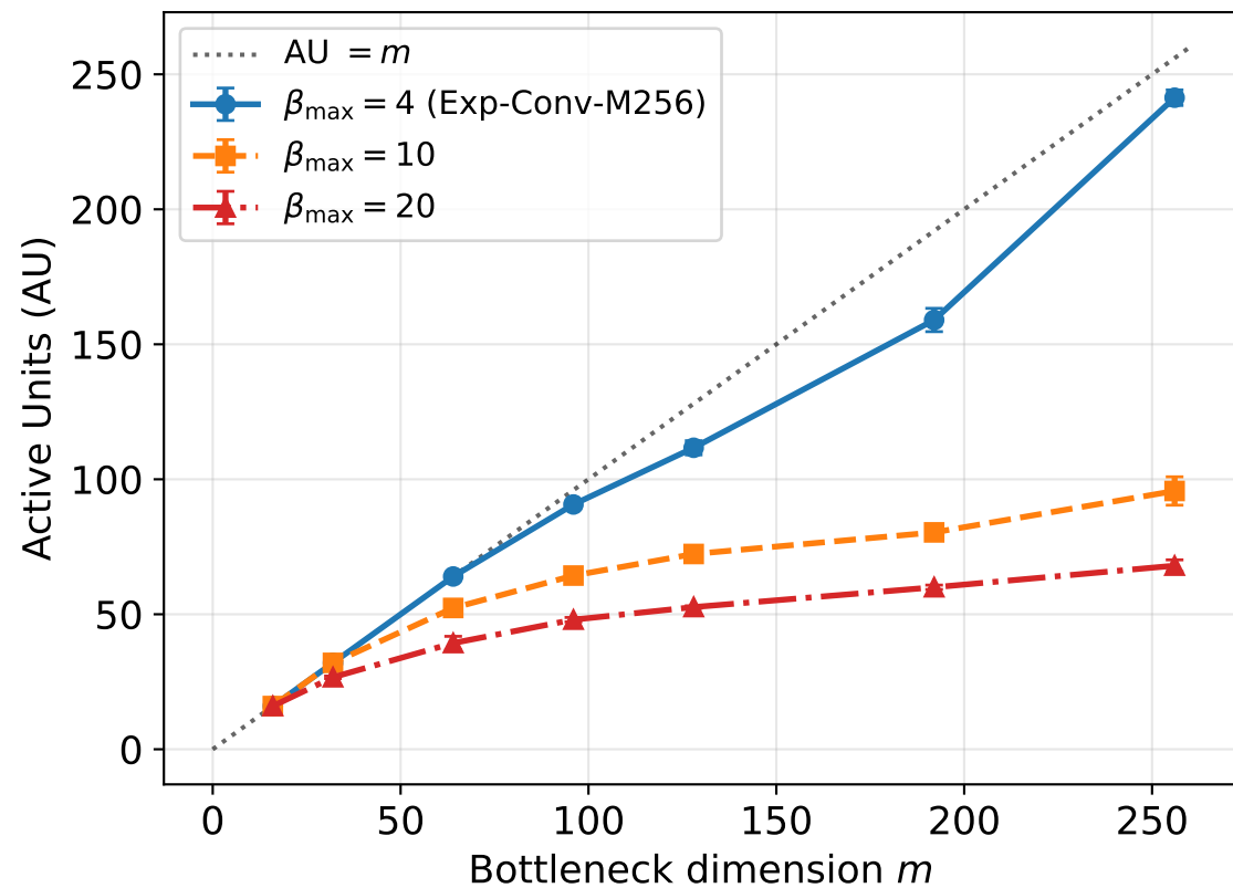
MNIST Conv-VAE: AU vs. m (mean \pm std, 3 seeds)
