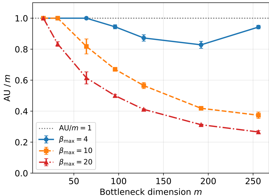
Active ratio AU/ m vs. m
