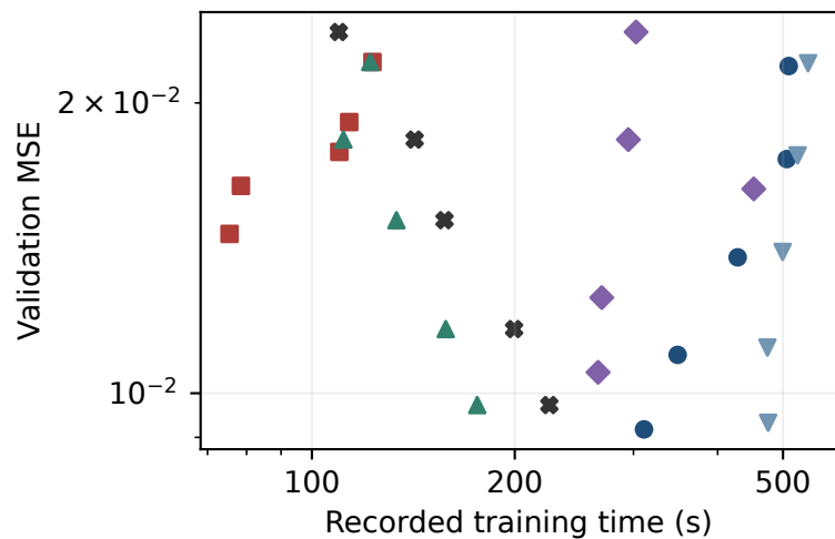
CIFAR-10
