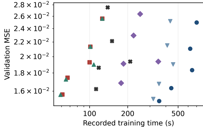
CIFAR-10
