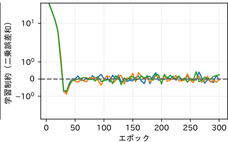
CIFAR-10
