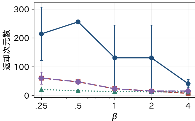
CIFAR-10
