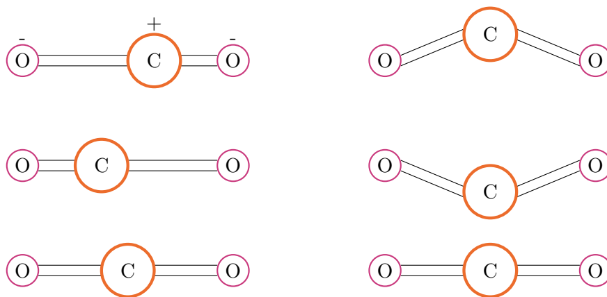
Figure 5.2: The two dipole moments of \text{CO}_2 that alter its dipole moment, thus making it a strong absorber/emitter in the infrared. Arrows indicate the movement of the central carbon molecule.
