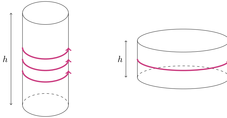
Figure 18.2: Intuition behind the Conservation of Potential Vorticity. When the fluid column gets stretched vertically (i.e., h increases), the fluid must rotate (magenta arrows ■) faster, and vice versa.
