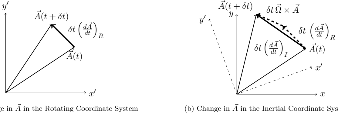
Figure 16.1: The change in \vec{A} in a rotating (16.1a) and inertial (16.1b) coordinate system. As seen in 16.1b, the change in the inertial coordinate system \delta t \left( \frac{d\vec{A}}{dt} \right)_I (thick arrow) is equal to sum of the change in the rotating coordinate system \left( \delta t \left( \frac{d\vec{A}}{dt} \right)_R \right) and the rotation of the rotating coordinate system \left( \delta t \vec{\Omega} \times \vec{A} \right) (thick dashed arrows).
