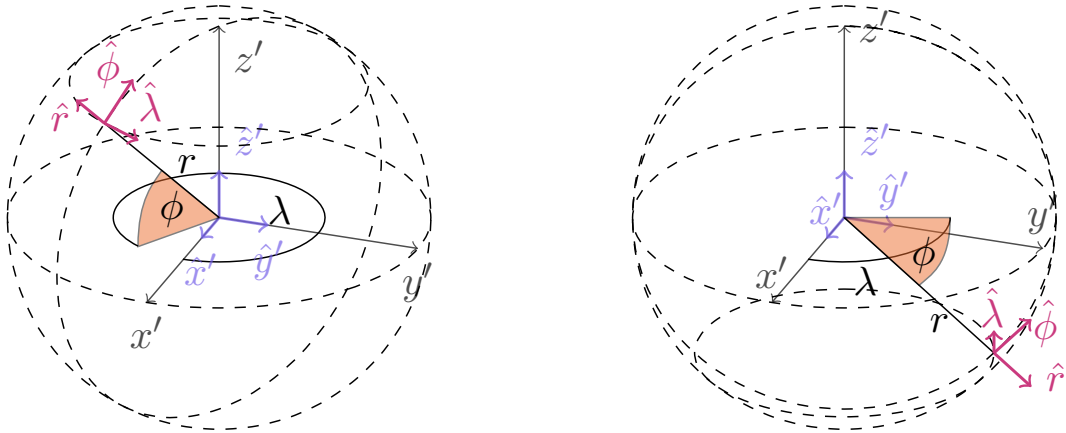
Figure 16.2: Spherical Coordinates. (x', y', z') indicate the directions of the basis vectors in the global cartesian coordinate system, while \hat{r}, \hat{\phi}, \hat{\lambda} indicate the basis vectors of the spherical coordinate system in magenta arrows. Compare the image on the left to the image on the right: as you can see, the spherical basis vectors (the magenta arrows) are space-dependent, and point in different directions depending on where you are on Earth (i.e., they depend explicitly on the position vector \vec{r} ).
