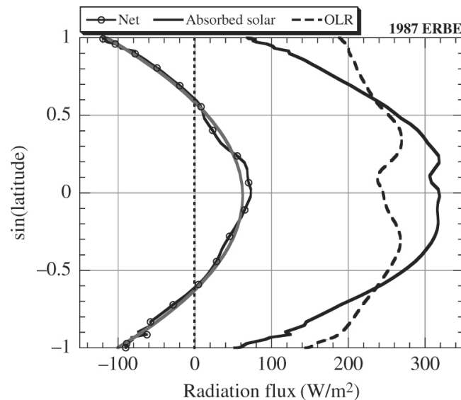
Figure 15.2: Figure from Ray’s book [3] showing differential heating. The equator absorbs more solar radiation than it emits while the poles emit more radiation than it absorbs. As such, to close the energy balance there must be a poleward energy transport by the atmospheres and oceans.
