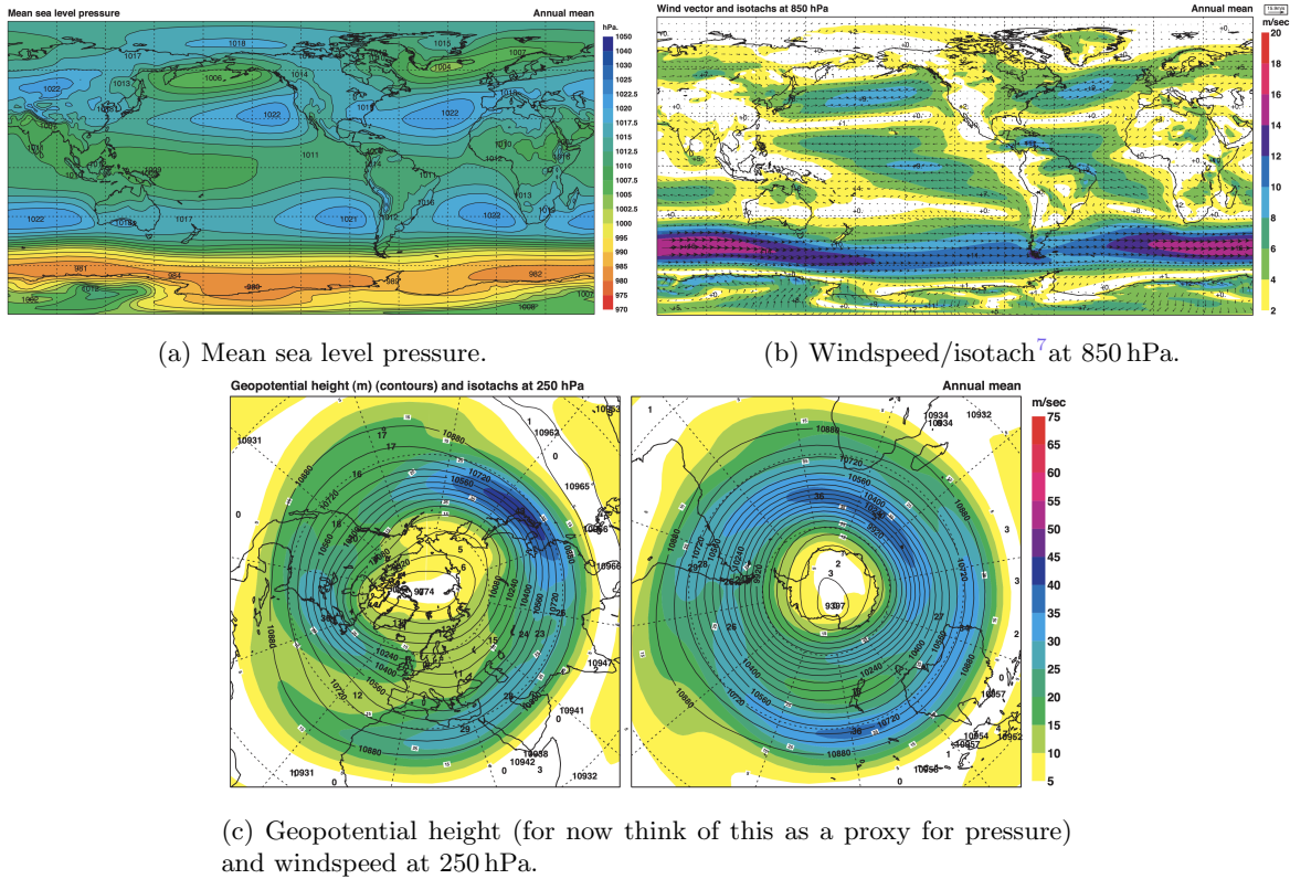
Figure 17.2: Annual Mean Renalysis Data from ERA40 [8] comparing pressure p_s (or geopotential height \Phi ) and horizontal wind speed \vec{u}_h . Geostrophic balance predicts that the direction of \vec{u}_h should be along isobars, and the magnitude of \vec{u}_h should scale with pressure gradients. The former is shown by figures 17.2a and 17.2b. Note that the colours should be slightly out of phase (as predicted by geostrophic balance) – focus instead on the arrows in figure 17.2b, which should blow along the blobs in figure 17.2a. The latter is shown by figure 17.2c, where the colours and contours should roughly line up. As you can see, though, there are clear deviations not only at the equator but at high latitudes too! We’re clearly missing something here.
