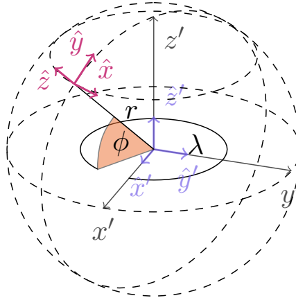
Figure 16.3: Local Cartesian Coordinates. (x', y', z') indicate the directions of the basis vectors in the global cartesian coordinate system, while \hat{x}, \hat{y}, \hat{z} indicate the basis vectors of the local cartesian coordinate system in magenta arrows.
