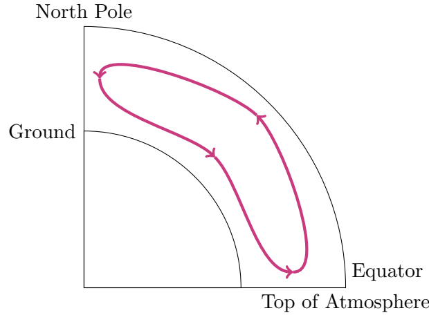
Figure 15.3: Hadley’s Convection Cell Model: heat is transported poleward by air parcels which are heated near the equator, rise, then flow poleward, before sinking and flowing southward to complete the loop. As the air parcels flow north/southward, they acquire a zonal velocity due to the rotation of the Earth.
