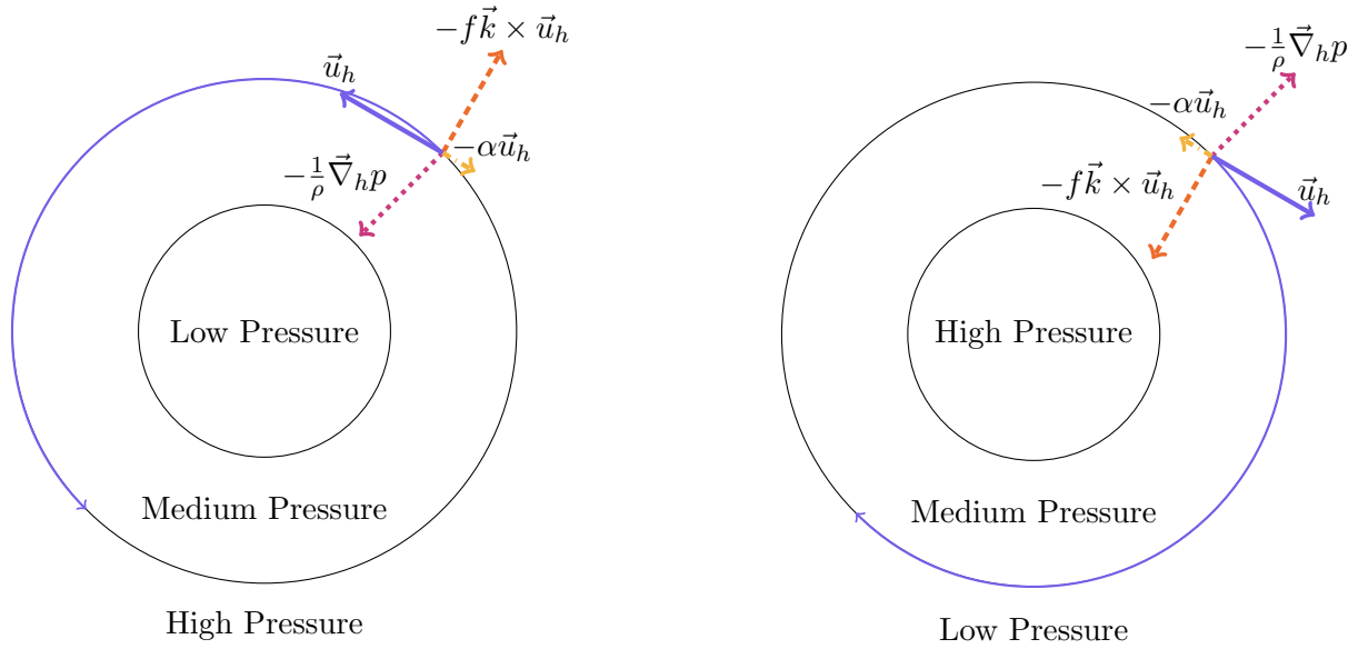
Figure 17.4: Cyclones and Anticyclones in the northern hemisphere ( f > 0 ) near the surface accounting for the effects of friction. Isobars are drawn as solid black lines ■, the pressure gradient force \left(-\frac{1}{\rho}\vec{\nabla}_h p\right) as thick dotted magenta arrows ■, the coriolis force \left(-f\vec{k} \times \vec{u}_h\right) as thick dashed orange arrows ■, the velocity (\vec{u}_h) as thick filled dark blue arrows ■, and the friction (-\alpha\vec{u}_h) as dash dotted yellow arrows ■.
