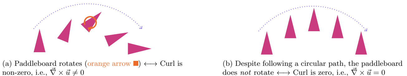
Figure 15.1: Paddleboard (magenta triangle \blacksquare ) demonstration of curl. The Dotted Blue Arrow \dashrightarrow indicates the direction of time evolution (the paddleboard is being advected by the velocity field \vec{u}(\vec{r}) ).
