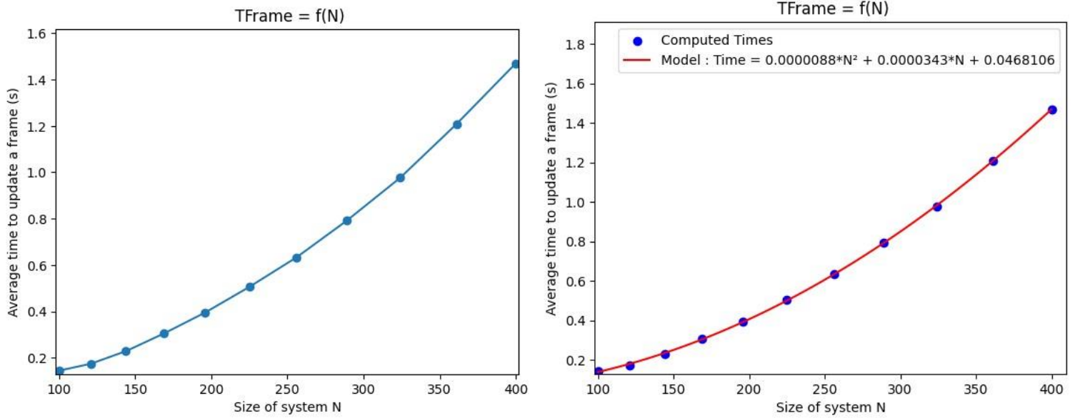
Fig. 7 & 8 : Time to update 1 frame, averaged over 100 frames, with (right) and without (left) polyfit model
