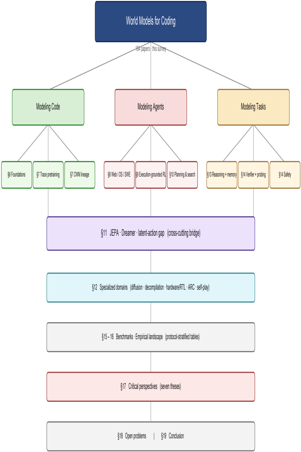
Figure 2: Taxonomy of world models for coding. The three primary modeling axes (code, agents, tasks) are bridged by the JEPA / Dreamer / latent-action discussion in §11. Specialized domains and synthesis chapters sit below.
