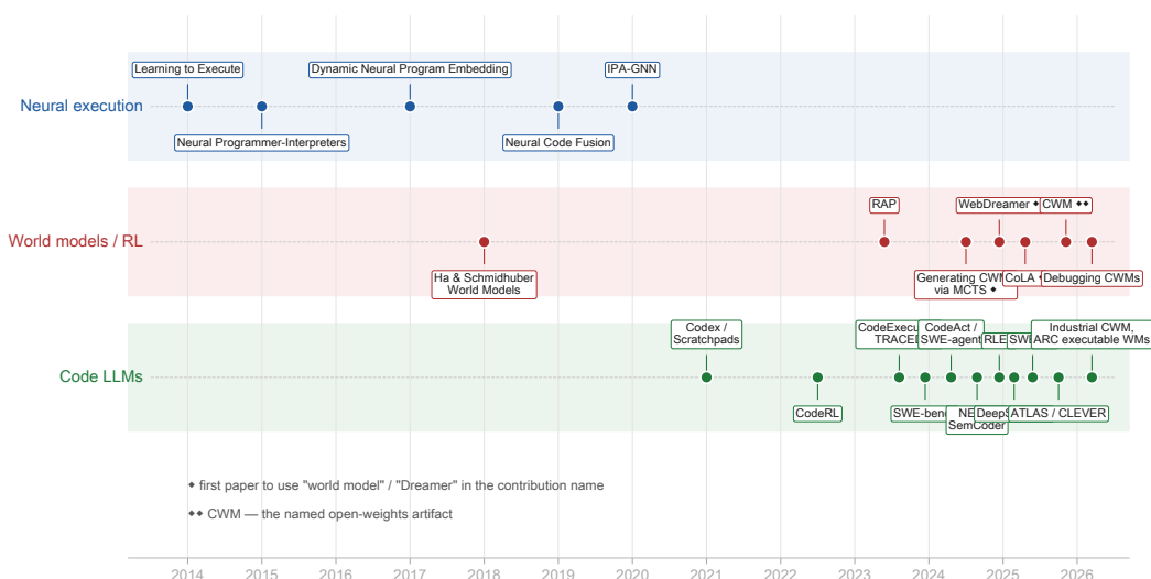
Figure 1: Twelve-year arc of code world models. Three parallel lineages — neural execution, world models / RL, and code LLMs — converge in 2025–2026 around the named artifact CWM. [?] marks the first paper to use “world model” / “Dreamer” in a contribution name; [?] marks CWM as the named open-weights artifact.
