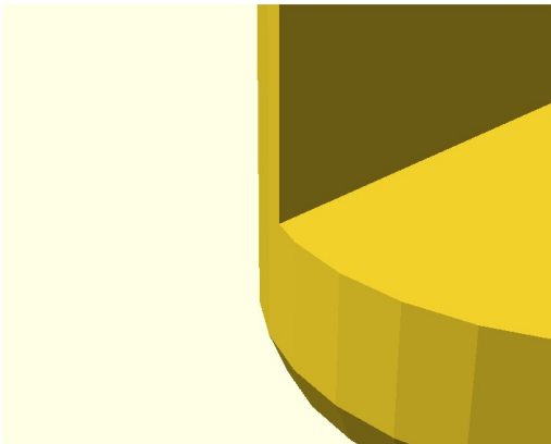
S6-T05 elbow_curved_endface [saddle=2 at stock (foot-clamped)] crease dies on a cylindrical end wall, 3 facets across VALID warnings=2
