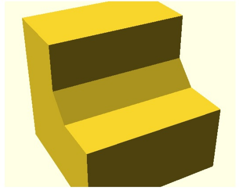
AC01-R2-C3 AC01 fn=8 chamfer fan folds=0 tube=0 capTri=0 cap=0 coons=0 saddle=0 flat=0 fan=2 weld=1 none=0 VALID warnings=0 OK
