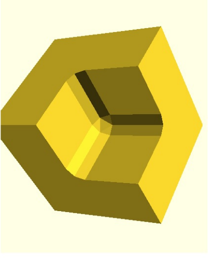
AC04-R2-C2 AC04 fn=8 fillet capTri folds=0 tube=0 capTri=1 cap=0 coons=0 saddle=0 filat=3 fan=0 weld=3 none=0 VALID warnings=0 OK
