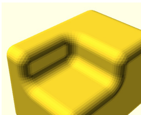
AC11-R4-C2 AC11 fn=32 fillet tube folds=0 tube=3 capTri=11 cap=0 coons=0 saddle=0 flat=0 fan=0 weld=26 none=0 VALID warnings=0 OK
