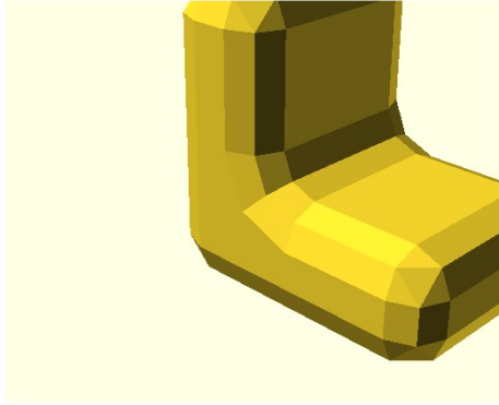
AC06-R2-C2 AC06 fn=8 fillet tube folds=0 tube=2 capTri=10 cap=0 coons=0 saddle=0 flat=0 fan=0 weld=16 none=0 VALID warnings=0 OK
