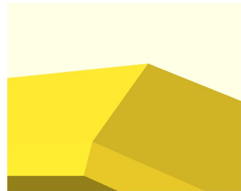
AC22-R3-C3 AC22 fn=19 chamfer fan folds=0 tube=0 capTri=0 cap=0 coons=0 saddle=0 flat=0 fan=8 weld=40 none=0 VALID warnings=0 OK
