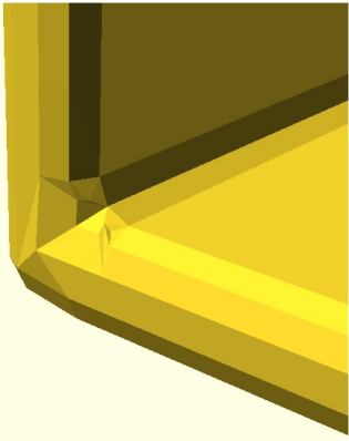
S6-T07 elbow_facet_endface [one of each: tube=1 coons=1] end face kinks 10deg exactly at the crease VALID warnings=0
