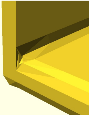
S6-T09 elbow_thin_arm [saddle+fan, turn seat (was torus tube=2)] arm 3 thick against 2R=4 VALID warnings=2
