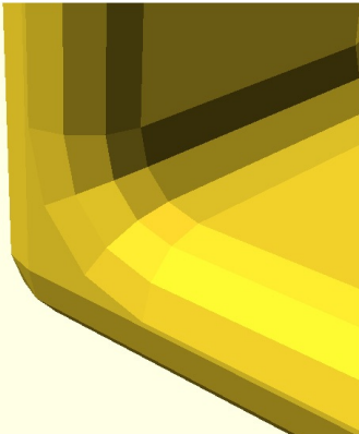
S6-T08 elbow_crowded [torus tube=2, not crowded out] arms 6 thick against 2R=5.8 VALID warnings=0
