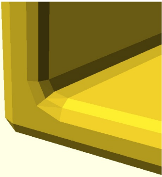
S6-T01 elbow_oblique75 [canal tube=2] end face raked 15deg, crease meets it at 75deg VALID warnings=0
