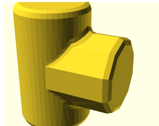
S5-T12 mixed_fn [centroid fan fan=4] 48/10-facet junction (5,0,10) warnings=0
