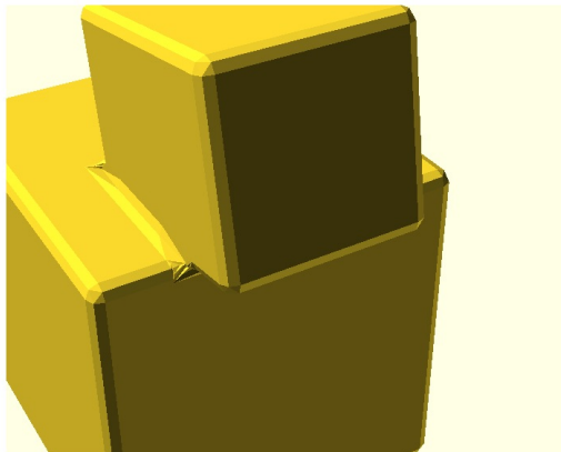
S5-T11 refused_neighbour [saddle saddle=6] refused crease (7.5,4,7.44) + built bead warnings=0
