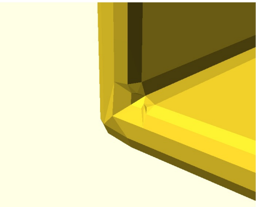
S6-T07 elbow_facet_endface [one of each: tube=1 coons=1] end face kinks 10deg exactly at the crease VALID warnings=0
