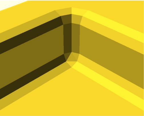
S6-T10 step_notch [torus + tri-cap tube=3 capTri=11] inverse elbow: 2 concave + 1 convex VALID warnings=0
