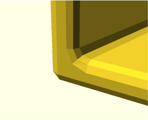
S6-T01 elbow_oblique75 [canal tube=2] end face raked 15deg, crease meets it at 75deg VALID warnings=0
