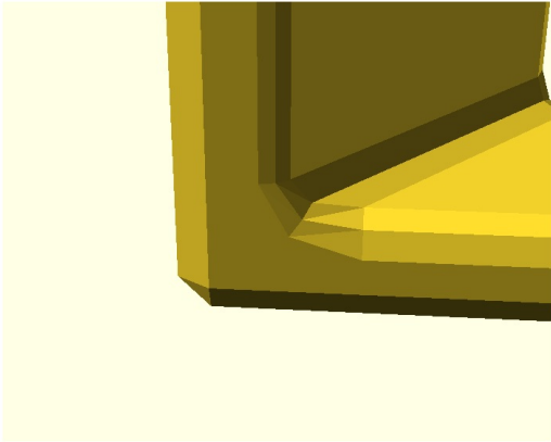
S6-T02 elbow_oblique50 [canal tube=2] end face raked 40deg, crease meets it at 50deg VALID warnings=0
