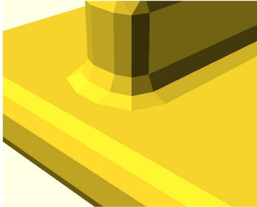
S5-T05 rib [torus + saddle tube=4 saddle=4] rib end on plate (20,2,5,2,5) warnings=0
