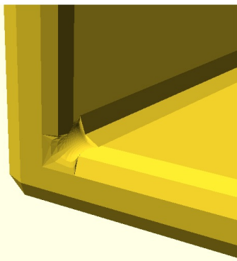
S6-T01 elbow_oblique75 [loft:oblique-face] end face raked 15deg, crease meets it at 75deg VALID warnings=0
