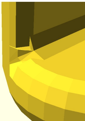
S6-T05 elbow_curved_endface [loft:curved-face] crease dies on a cylindrical end wall, 3 facets across VALID warnings=0
