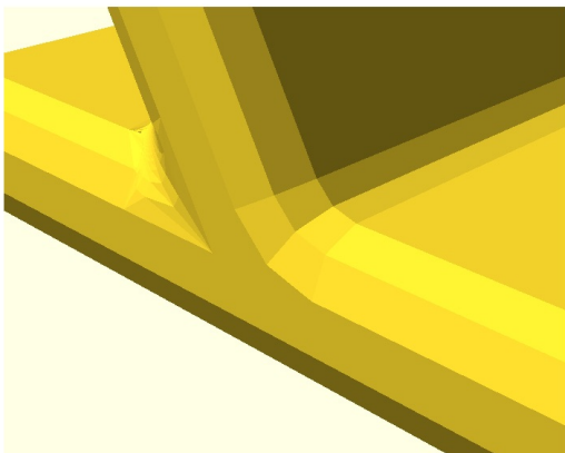
S6-T04 elbow_dihedral120 [loft:non-square] 120deg trough (leaning wall), square end face VALID warnings=0
