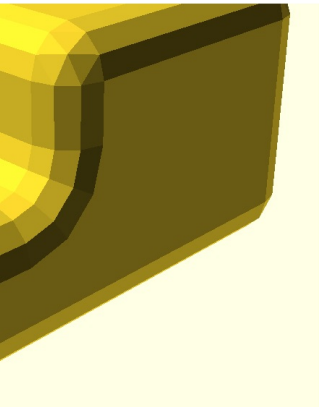
S5-T04 box_step [torus] back elbow (24,40,10) mirrored warnings=0
