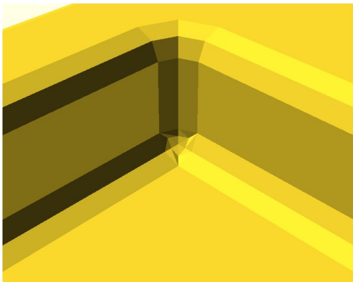
S6-T10 step_notch [loft:inverse] inverse elbow: 2 concave + 1 convex VALID warnings=0
