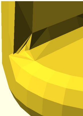
S6-T05 elbow_curved_endface [saddle=2 at stock (foot-clamped)] crease dies on a cylindrical end wall, 3 facets across VALID warnings=0
