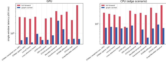
Figure 9. Single-window latency with and without graph-embedding caching, on GPU and CPU (log scale).
