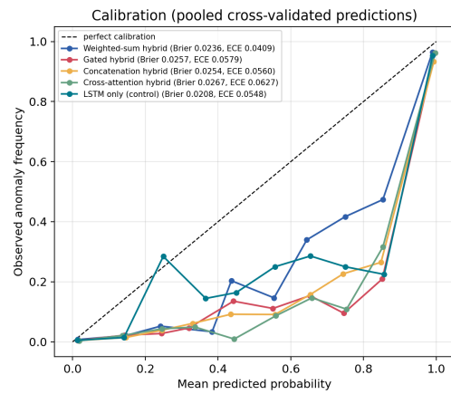
Figure 8. Reliability diagram from pooled cross-validated predictions.
