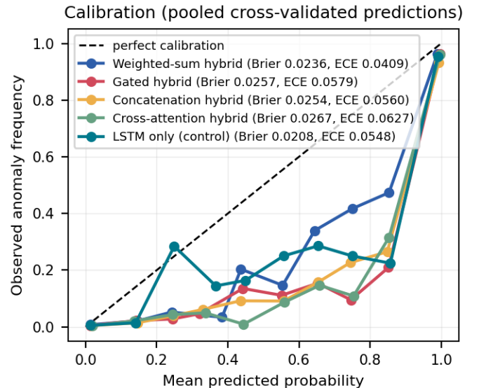
Figure 9. Reliability diagram from pooled cross-validated predictions.
