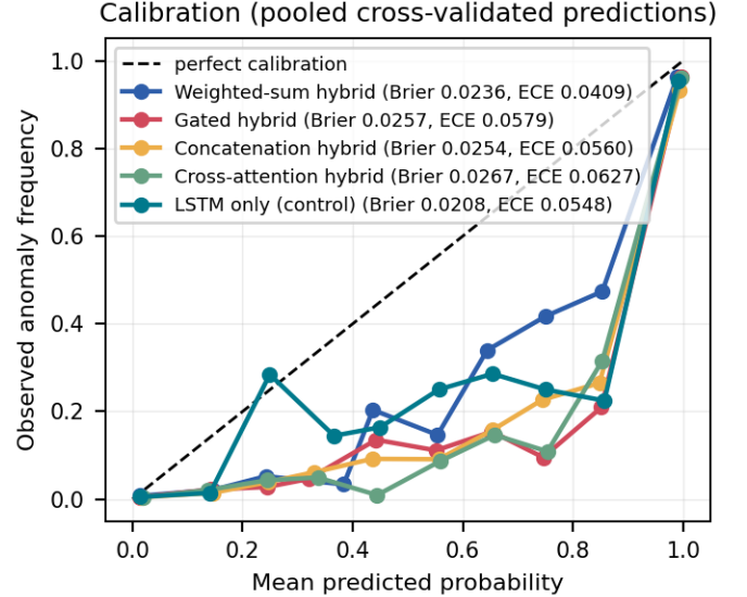
Figure 8. Reliability diagram from pooled cross-validated predictions.
