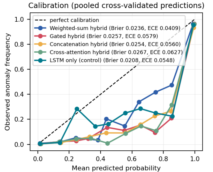
Figure 8. Reliability diagram from pooled cross-validated predictions.
