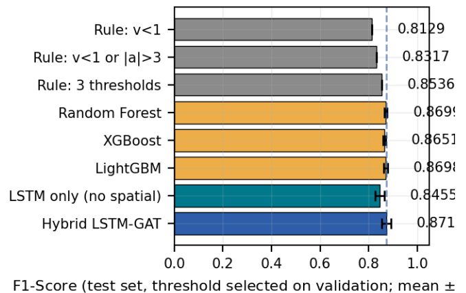
Reference points: rule-based and classical models
