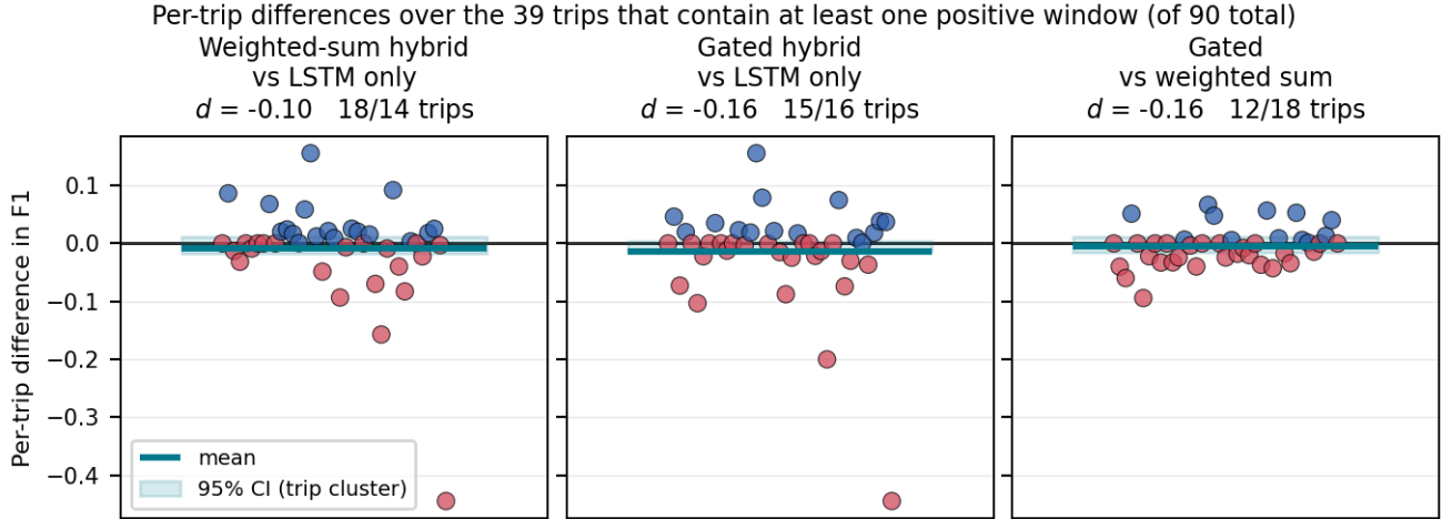
Figure 7. Per-trip differences in F1 for the three principal comparisons, over the 39 trips that contain at least one positive window. Each point is one trip; the horizontal band is the trip-level cluster-bootstrap interval for the pooled difference. The differences are centred near zero with trips falling on both sides, and each comparison has one trip whose difference is an order of magnitude larger than the rest.
