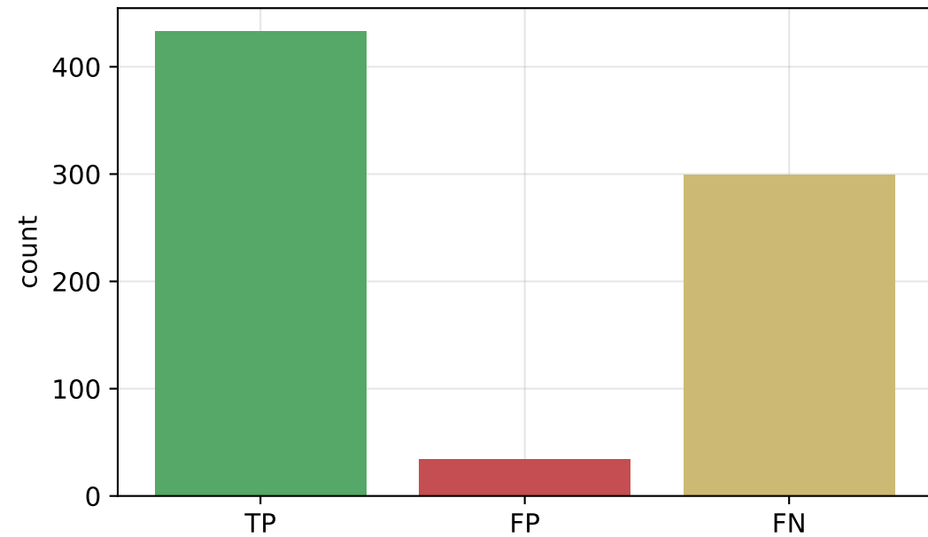
Detection totals
