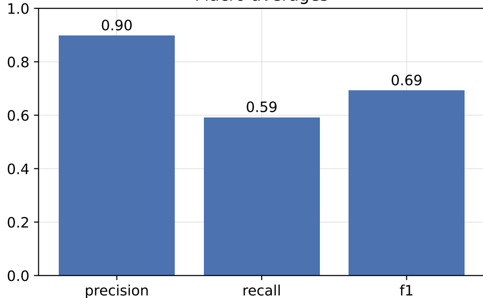
Macro averages
