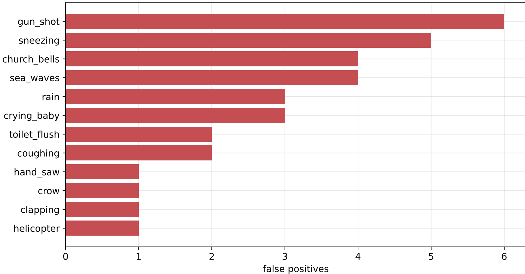
Top false-positive classes - v3.0
