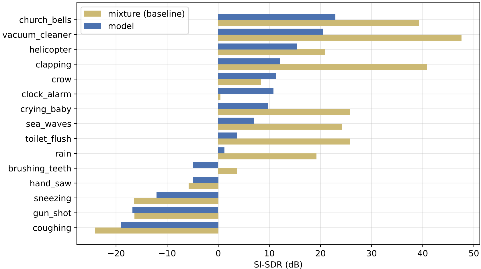
SI-SDR: mixture vs model - v3.0
