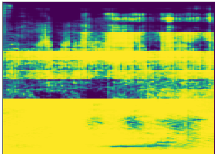
predicted mask
