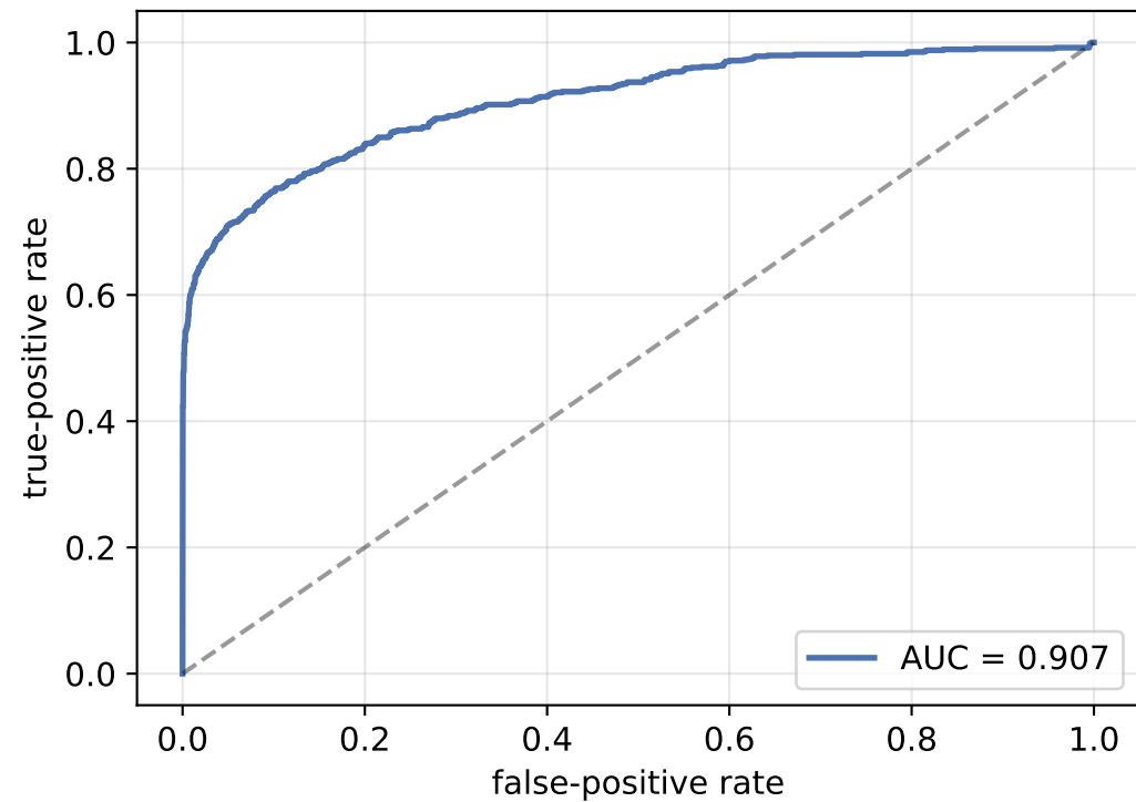
ROC (micro)
