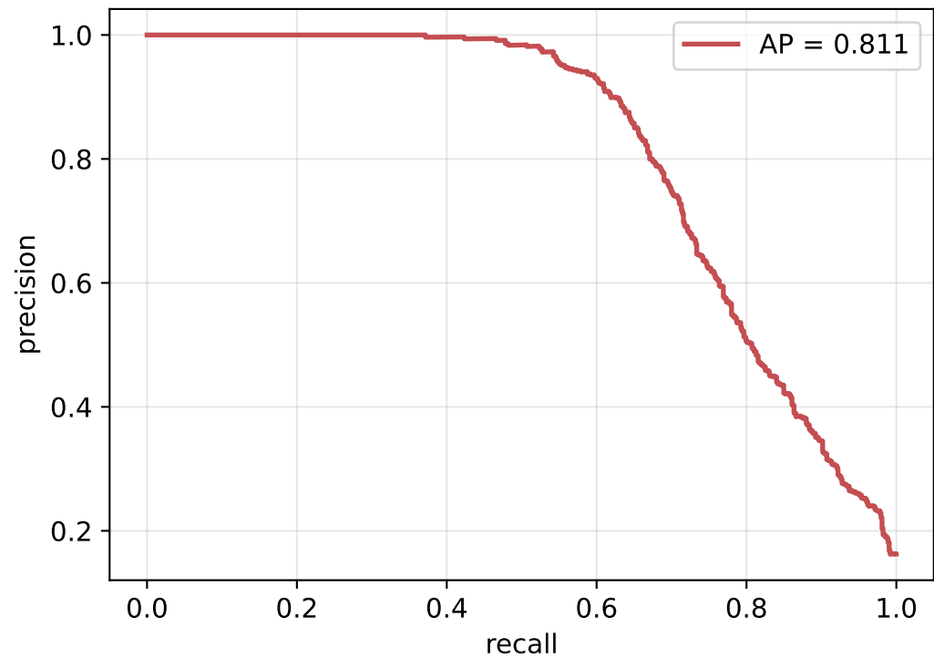
Precision-Recall (micro)
