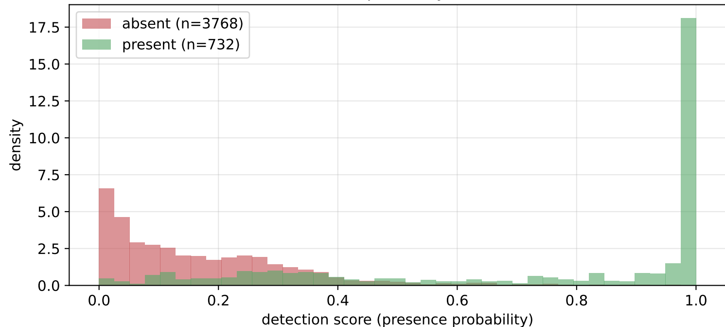
Score separability - v3.0
