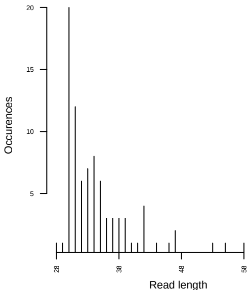
Single-end read length distribution
