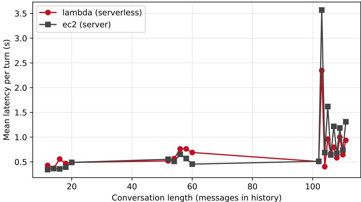
Latency vs. conversation length
