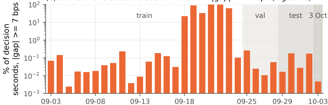
(b) Share of one-second decision rows with |\text{gap}| \geq 7 bps (log scale)
