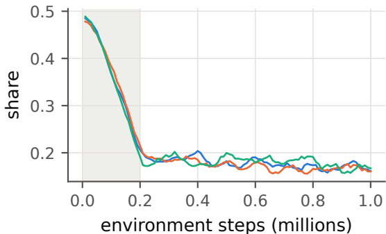
(c) Double DQN: share of screened entries taken
