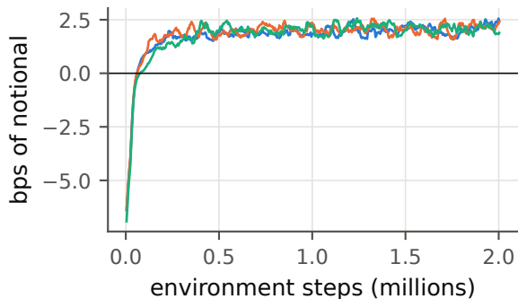
(b) PPO, 450 ms: training reward per window
