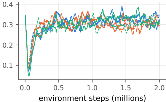
(a) share of screened entries taken
