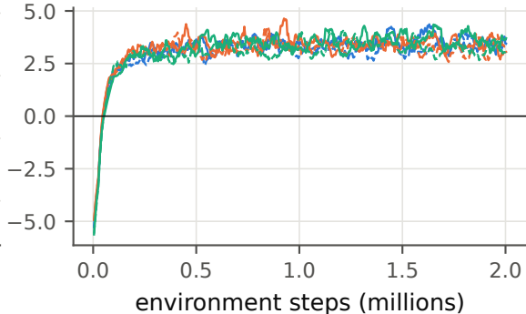
(b) training reward per window (bps)
