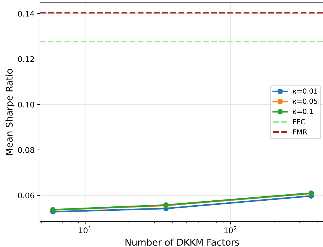
(a) Sharpe Ratios - KP14
