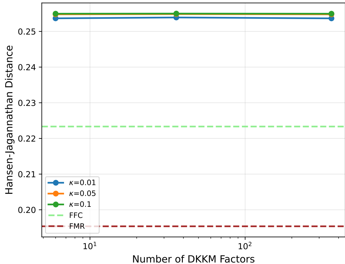
(b) HJ Distances - KP14
