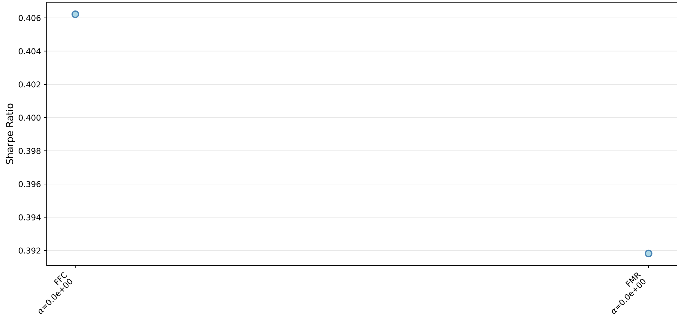
GS21 - Fama Sharpe Ratios (Distribution Across Panels)
