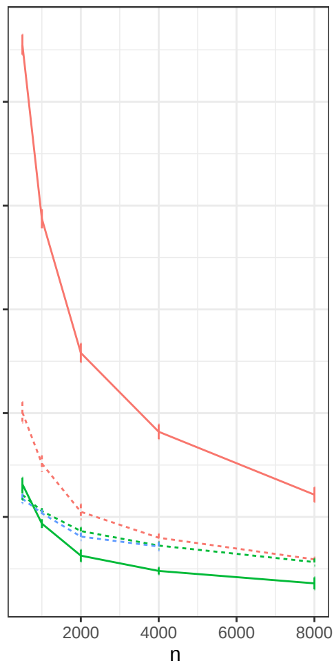
data ( \hat{\Sigma}_C )
