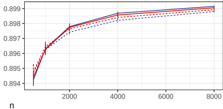
data ( \hat{\Sigma}_E )
