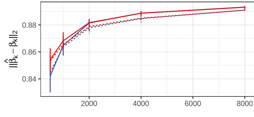
data ( \hat{\Sigma}_G )
