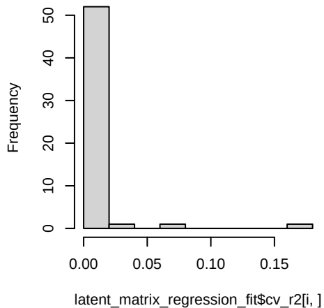
Histogram of latent_matrix_regression_fit$cv_r2[i, ]
