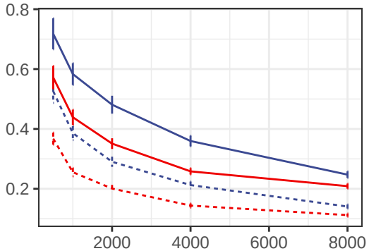
data ( \hat{\Sigma}_E )
