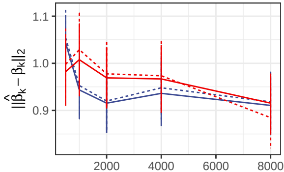
data ( \hat{\Sigma}_G )
