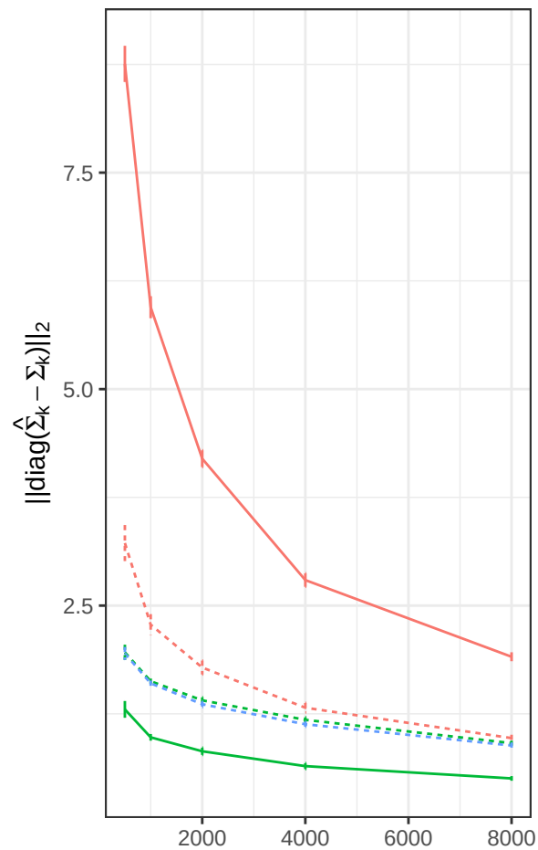
data ( \hat{\Sigma}_G )
