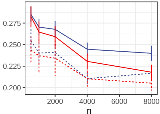
data ( \hat{\Sigma}_C )
