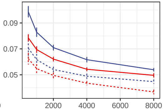
data ( \hat{\Sigma}_E )
