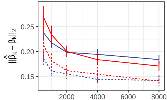
data ( \hat{\Sigma}_G )
