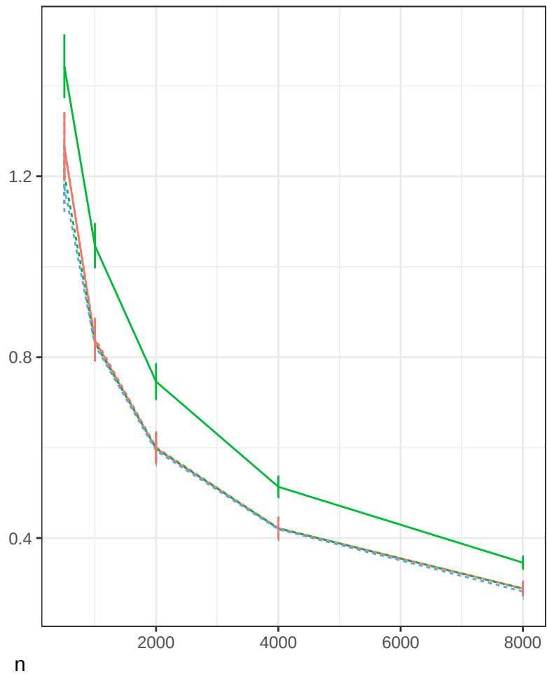
data ( \hat{\Sigma}_E )
