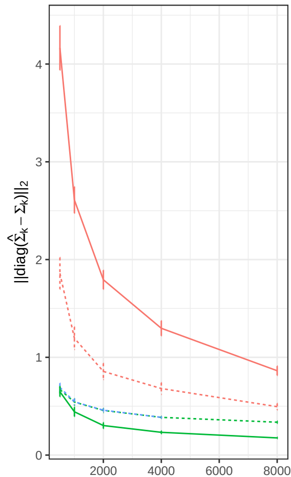
data ( \hat{\Sigma}_G )
