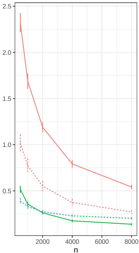
data ( \hat{\Sigma}_C )
